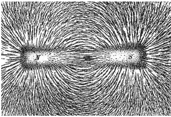
Fig. 9. Magnetic lines of force.
